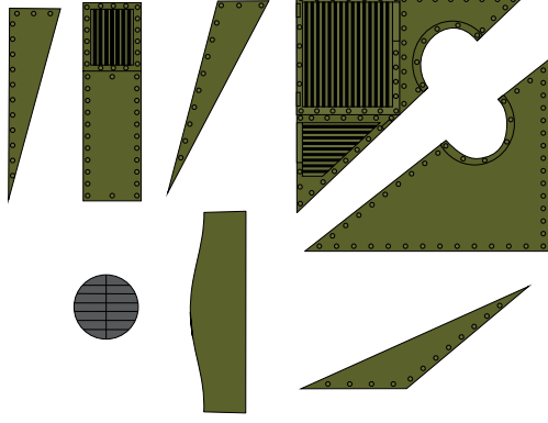
ENGINE'S COVER
